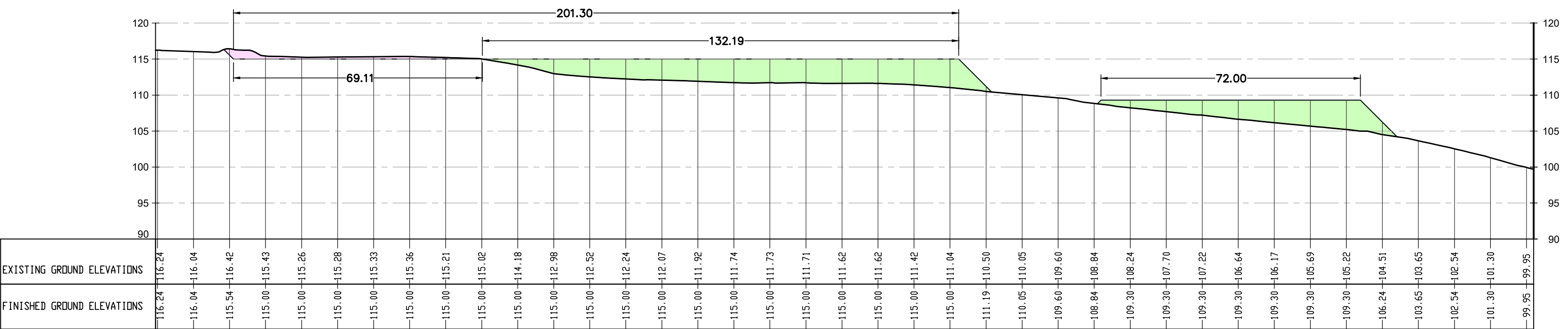
SECTION 6-6
